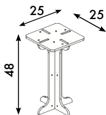
Tabouret simple
